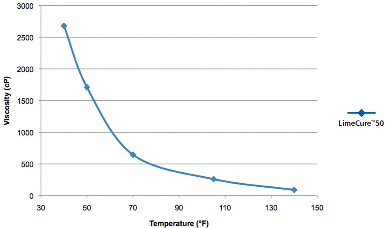
LimeCure™ 50 Viscosity vs. Temperature
